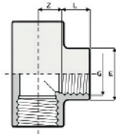
T12 90° Tee with BSP threaded female ends
