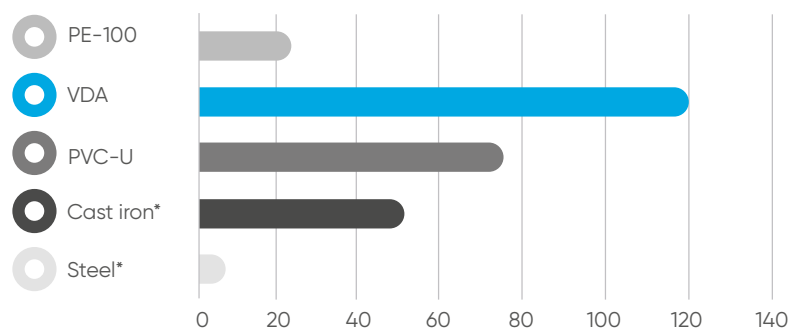
Installation rate m/h
