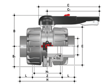
VKDIC DUAL BLOCK® 2-way ball valve with female ends for solvent welding, metric series
