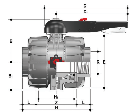
VKDFC DUAL BLOCK® 2-way ball valve with BSP threaded female ends
