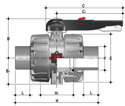
VKDDC DUAL BLOCK® 2-way ball valve with male ends for solvent welding, metric series
