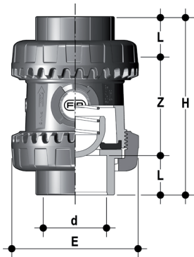
SSEIC - Hastelloy Spring Easyfit spring check valve with female ends for solvent welding, metric series
