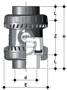
SSEIC True Union Spring Check Valve Easyfit with metric plain socket ends for solvent welding
