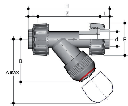
RVUAC Sediment strainer with female union ends for solvent welding, ASTM series
